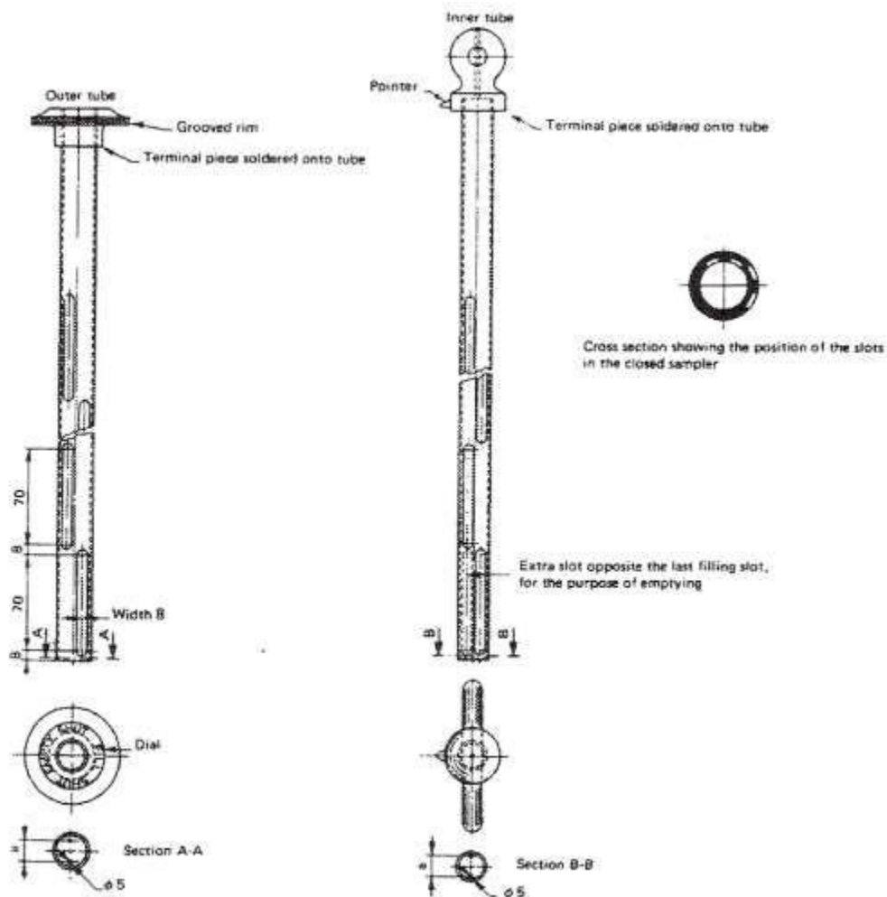
Figure 2 – Example of sampling tube (5.3.1) (Dimension for guidance only)
