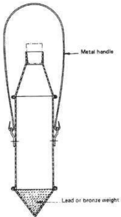
Figure 4 – Example for weighted bottle for sampling from tanks (6.3.2.1)
