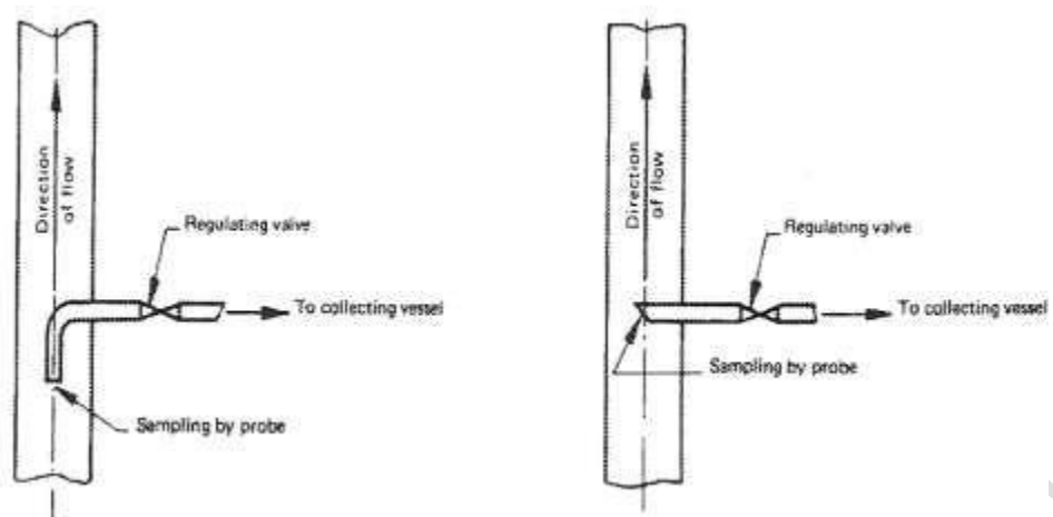
Figure 1 – Example of tapping sampler (4.2.2.1)
