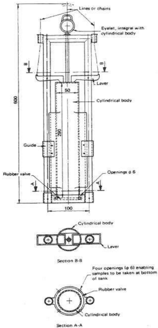
Figure 3 – Example of open ended cylindrical sampler (6.2.2.1) (Dimensions for guidance only)
